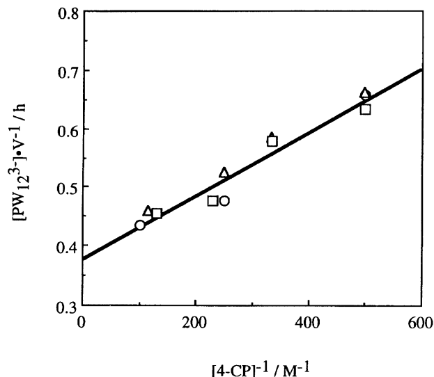
Fig. 8. Plot of 1/\text{rate} ( M s^{-1} ) versus 1/[4-CP] . The symbols refer the same as in Fig. 7.
