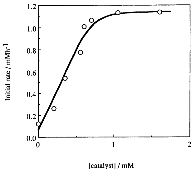
Fig. 6. Dependence of the catalytic activity for 4-chlorophenol photodecomposition by PW_{12}^{3-} on the catalyst concentration. [4-CP] = 2.0 mM; pH was adjusted at 1.0 with HClO_4 .
